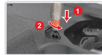
Push down the screw with flat head driver, then turn 90 degree counter clock-wise.
