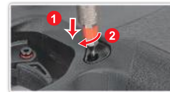
Push down the screw with flat head driver, then turn 90 degree clock-wise to lock.
